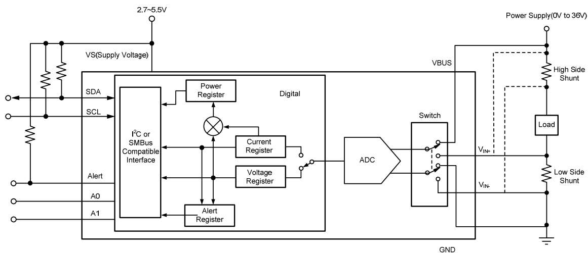
Figure 1 Function block diagram
